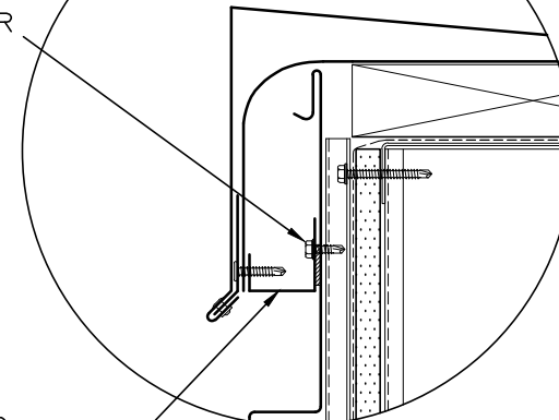
DETAIL AT MX 3.0 PANEL ( AT 6" REVEALL )
