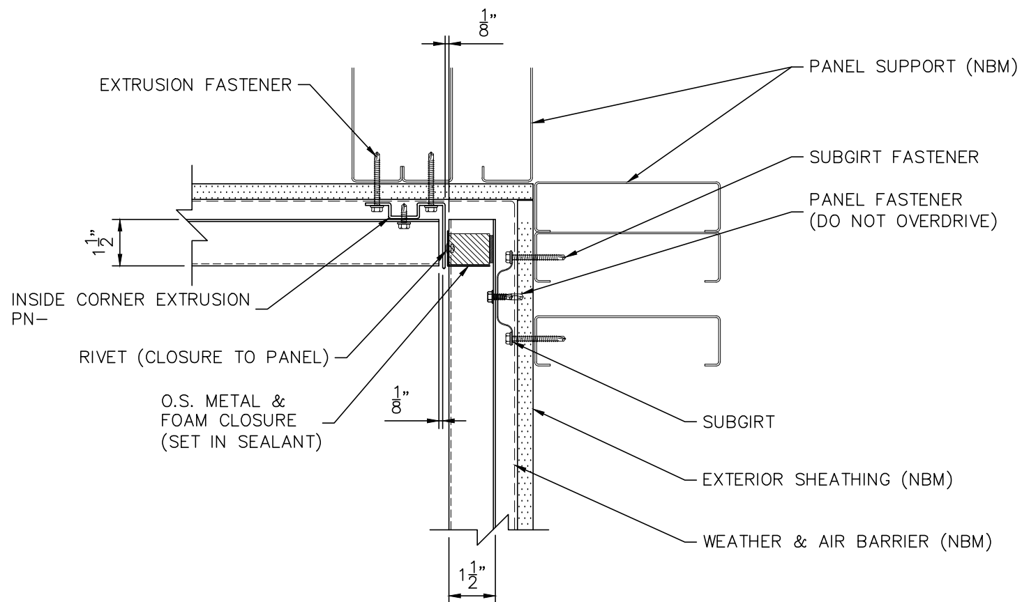
INSIDE CORNER DETAIL (w/ EXTRUSION)
