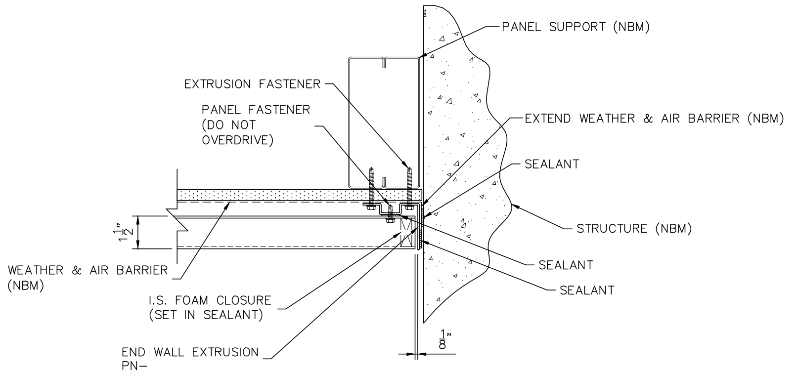
END WALL DETAIL
