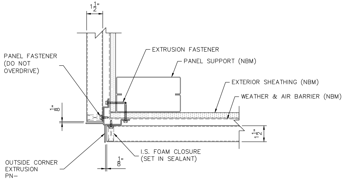
OUTSIDE CORNER DETAIL (w/ EXTRUSION)
