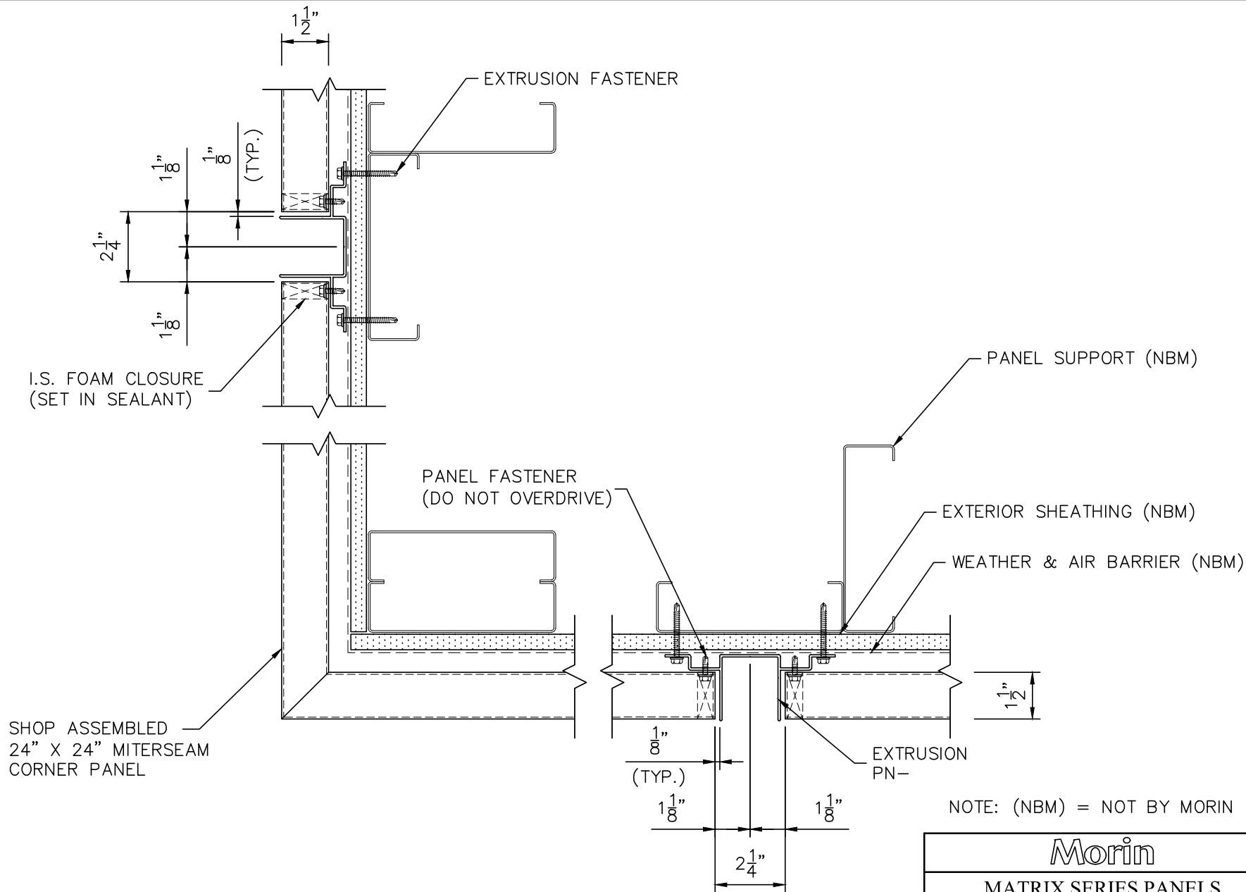
OUTSIDE CORNER DETAIL (w/ MITERSEAM)
