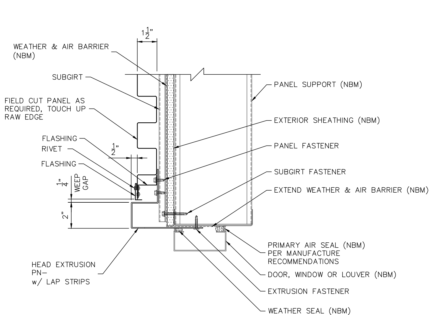
DOOR/WINDOW/LOUVER HEAD DETAIL
