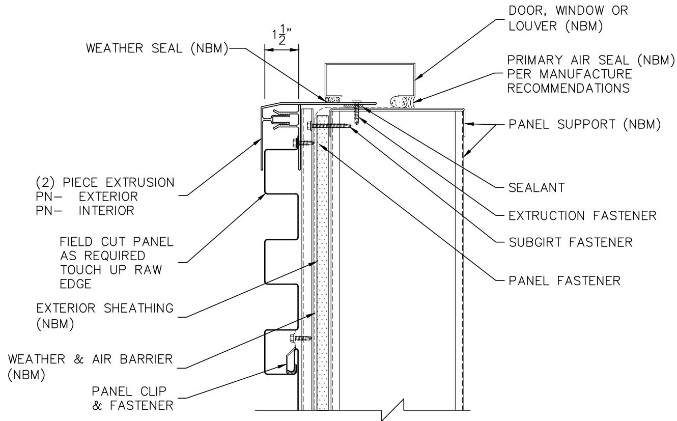
DOOR/WINDOW/LOUVER SILL DETAIL
