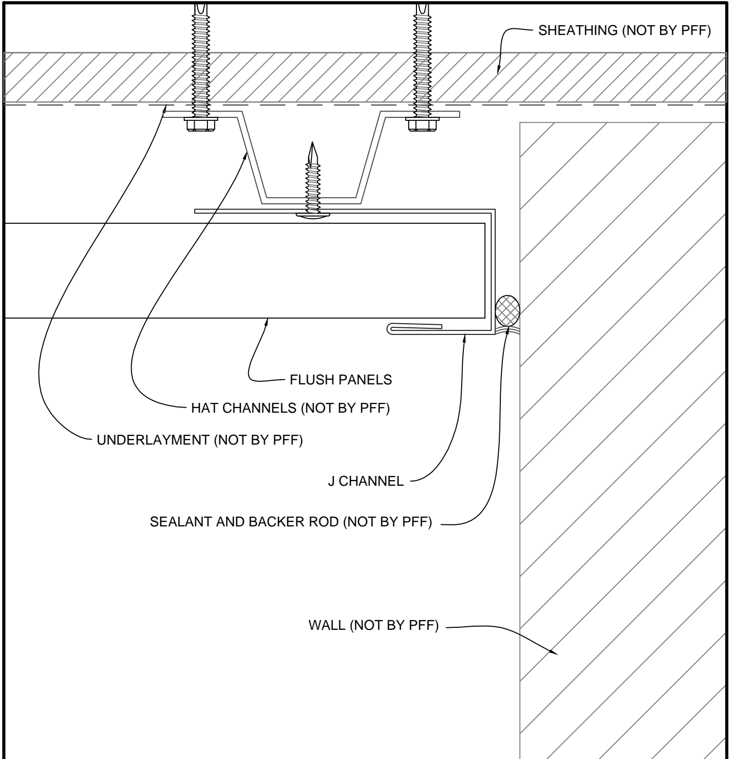
HORIZONTAL FLUSH PANELS - DETAIL F
