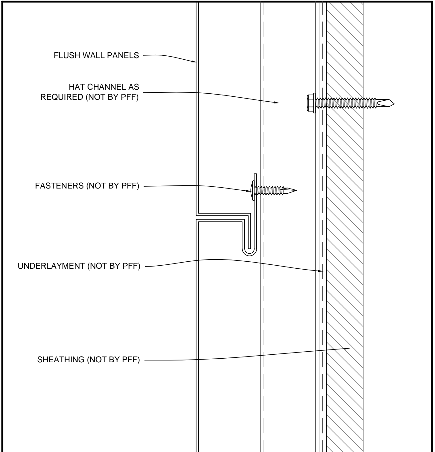
HORIZONTAL FLUSH PANELS - DETAIL A
