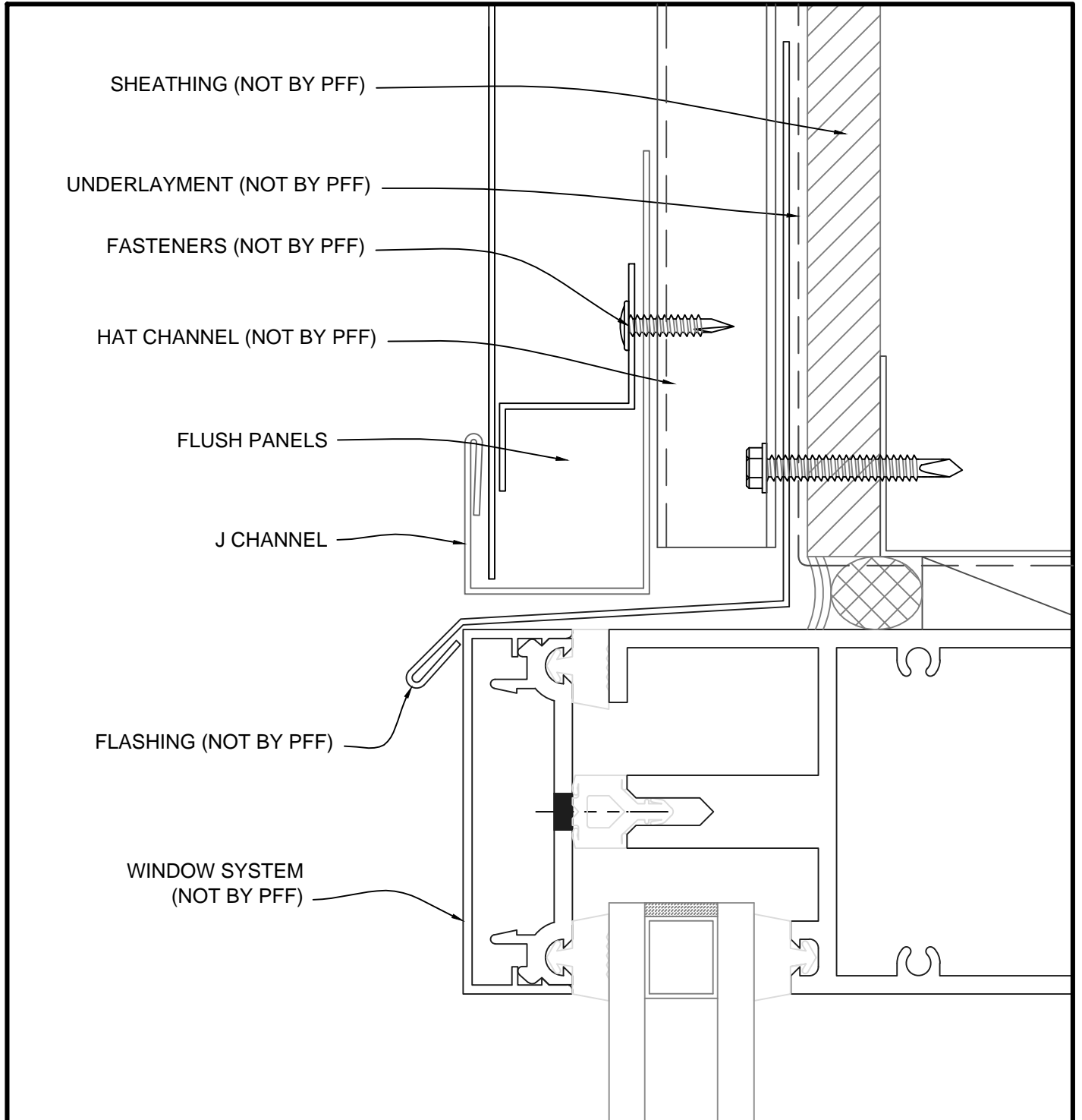
HORIZONTAL FLUSH PANELS - DETAIL K
