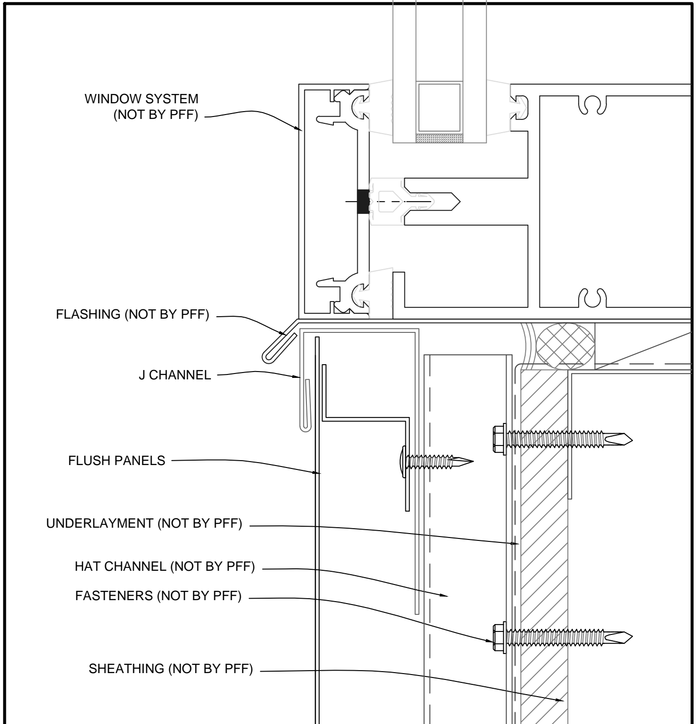
HORIZONTAL FLUSH PANELS - DETAIL L
