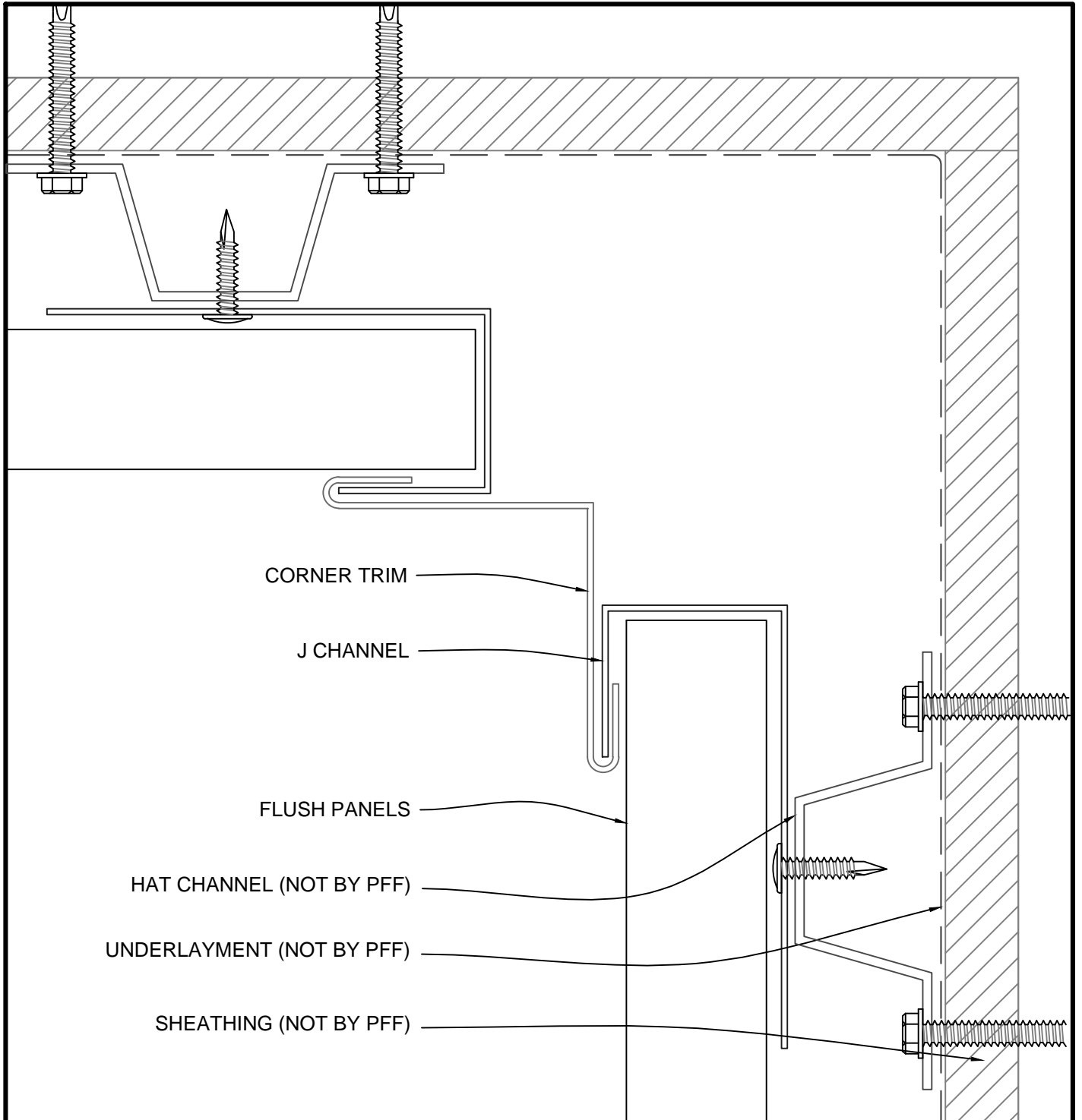
HORIZONTAL FLUSH PANELS - DETAIL E
