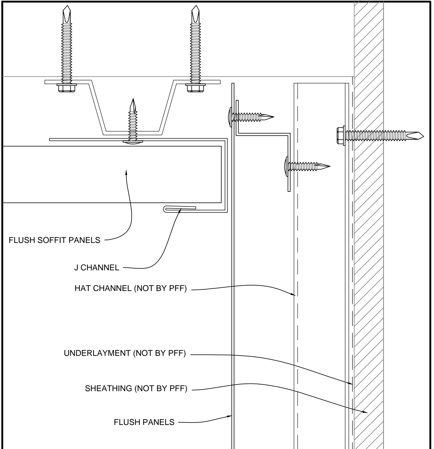
HORIZONTAL FLUSH PANELS - DETAIL H
