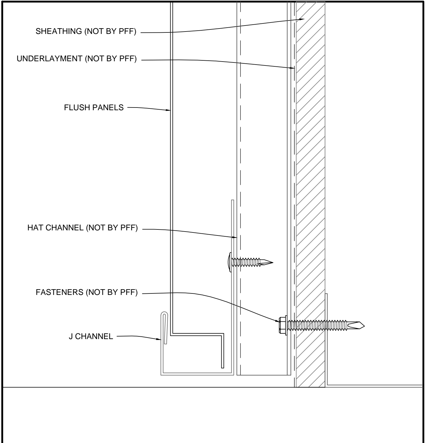
HORIZONTAL FLUSH PANELS - DETAIL C
