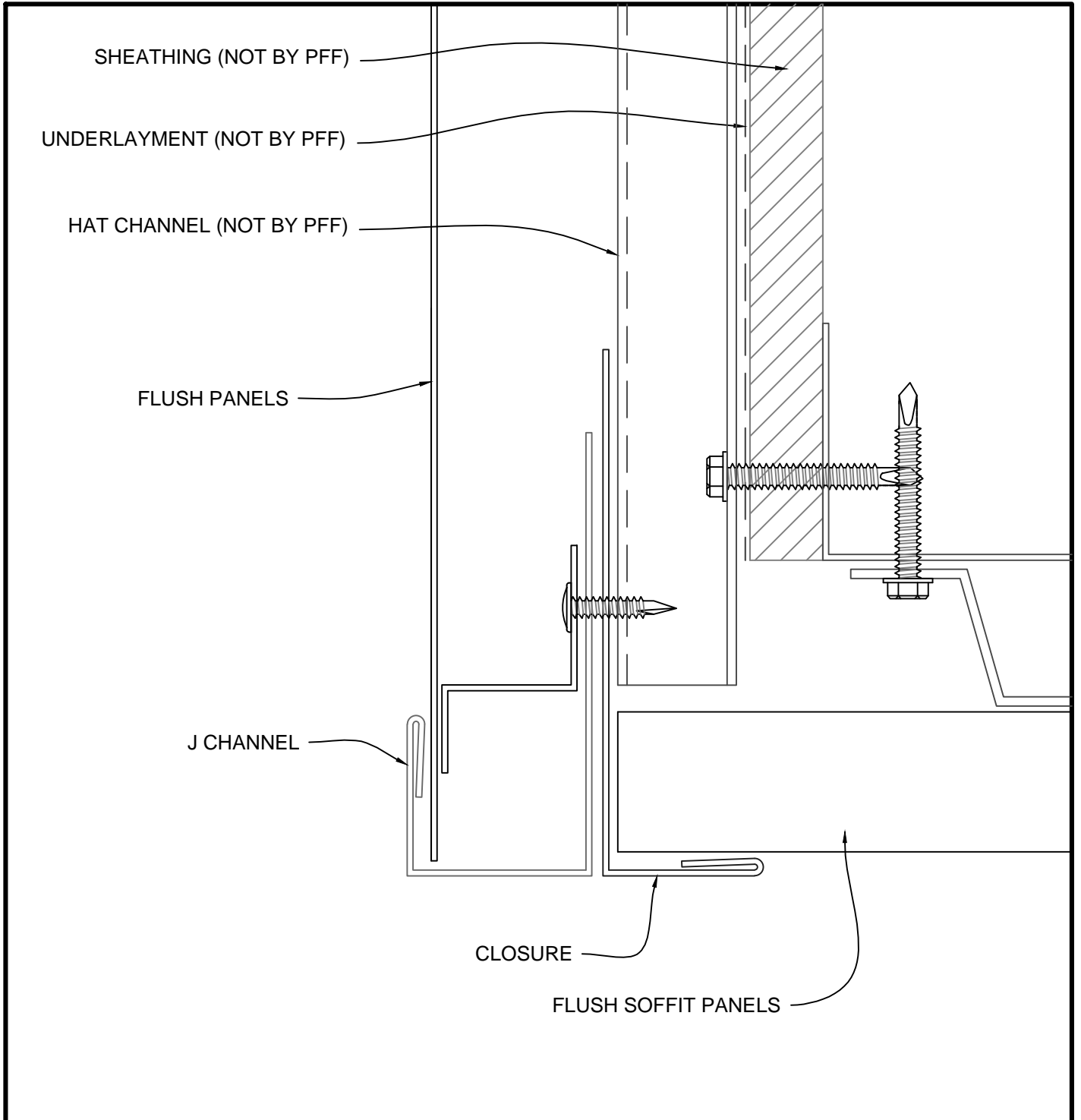
HORIZONTAL FLUSH PANELS - DETAIL G
