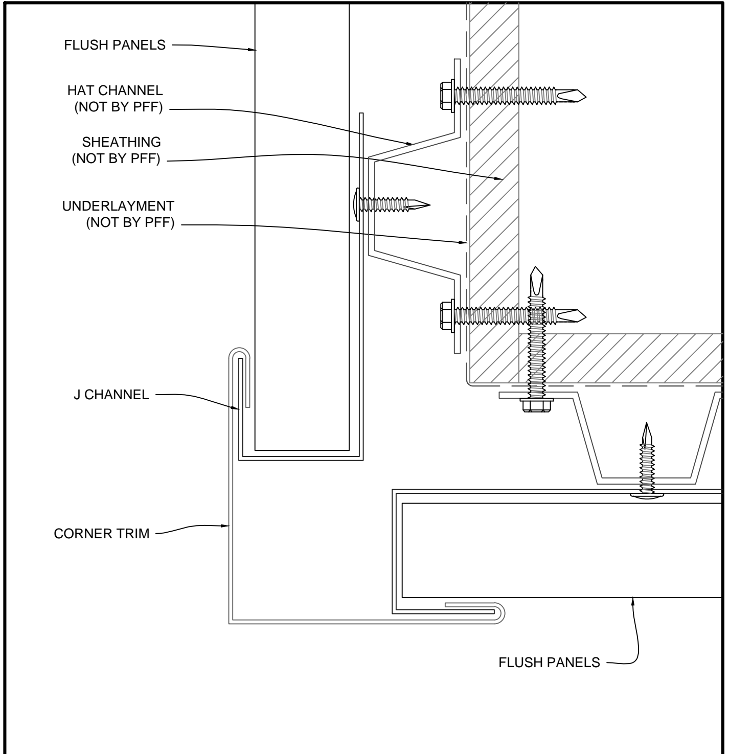
HORIZONTAL FLUSH PANELS - DETAIL D
