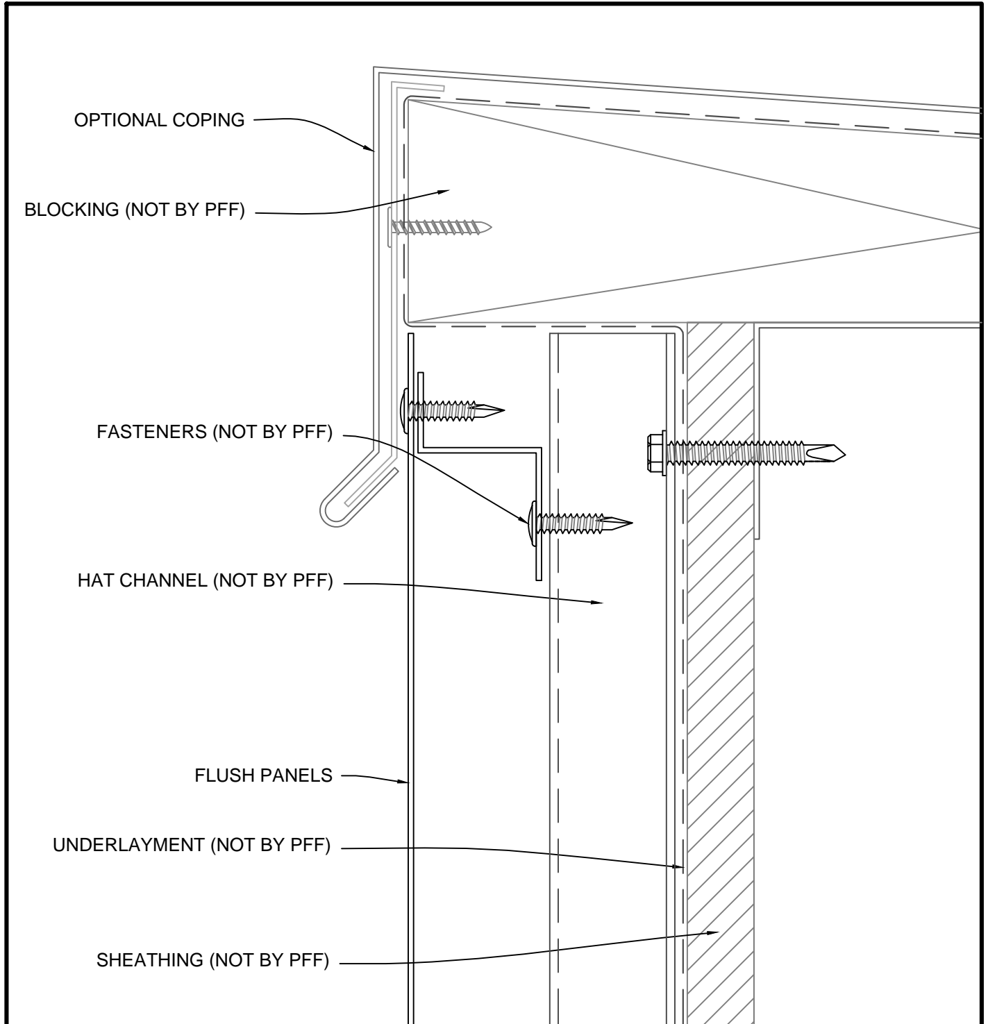
HORIZONTAL FLUSH PANELS - DETAIL B
