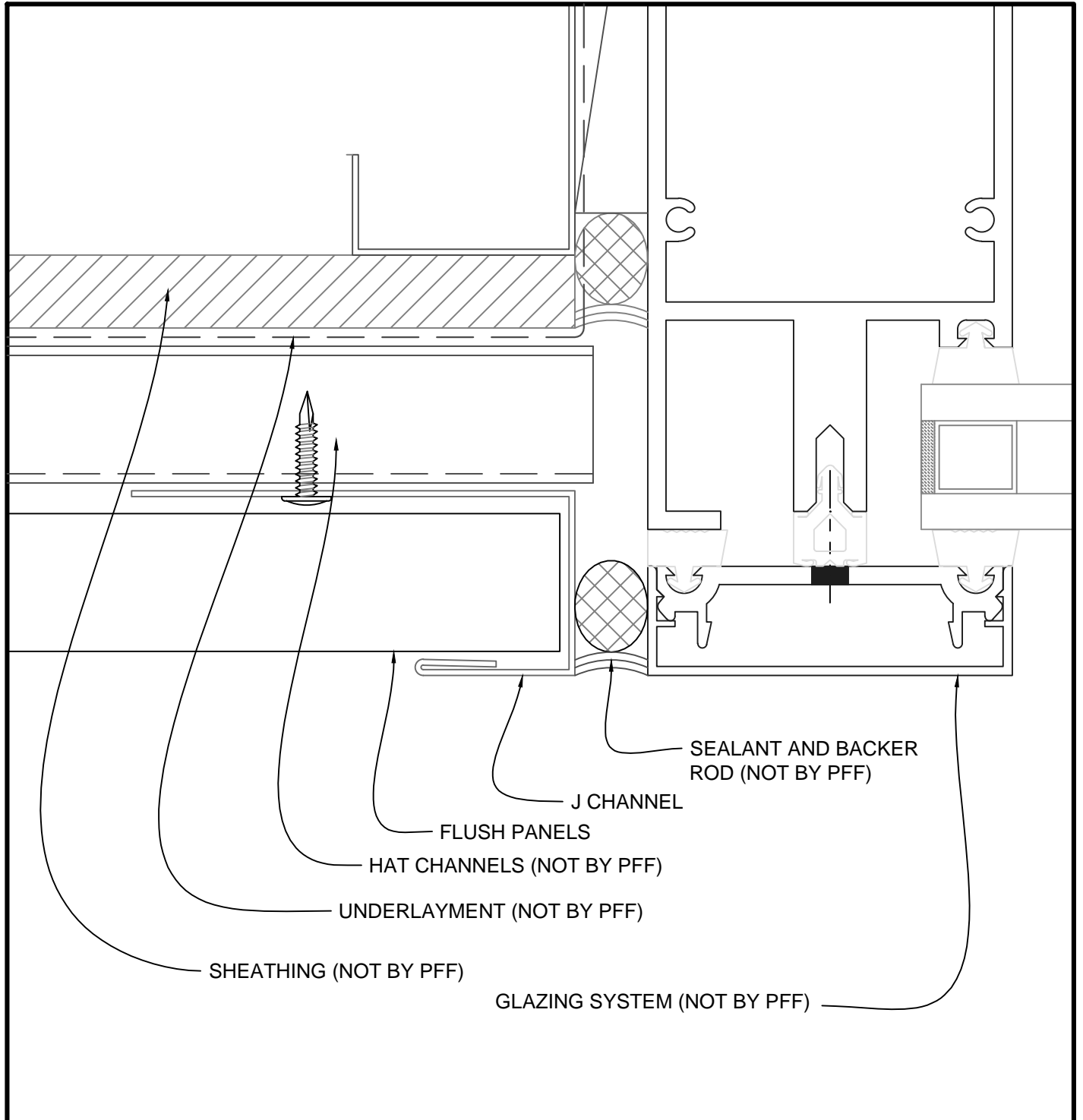
HORIZONTAL FLUSH PANELS - DETAIL J
