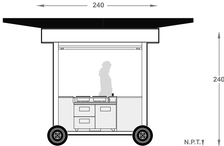
Vista frontal
