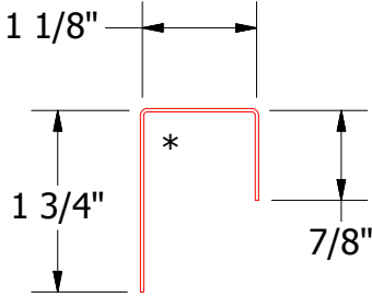
MCA118-J Channel
