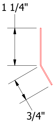
MFA995-Starter Cleat
