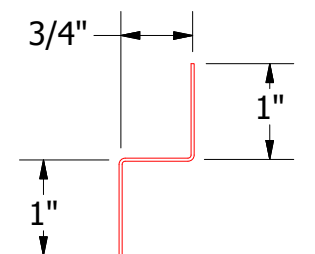
MCA681-Support Z
