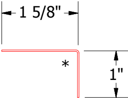
MCA680-Angle Trim
