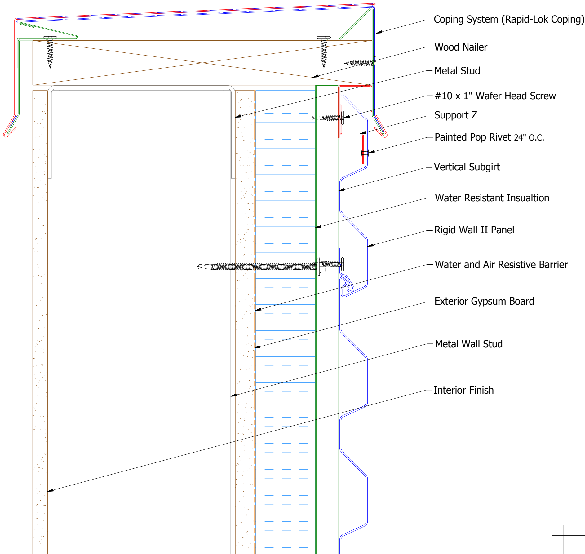
MCA681-Support Z
