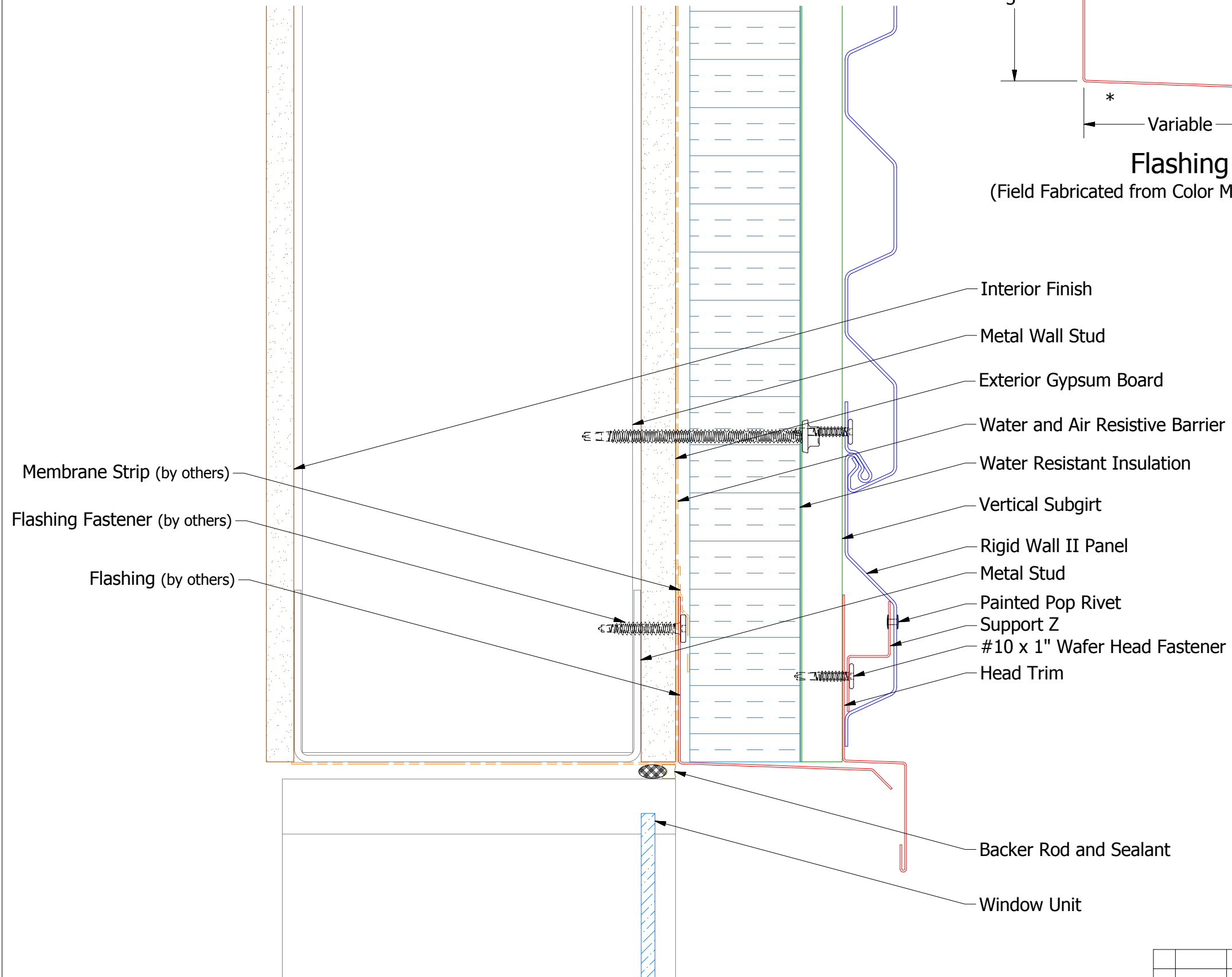
MCA550-Head Trim
