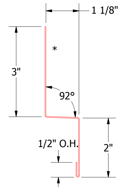
MCA550-Head Trim
