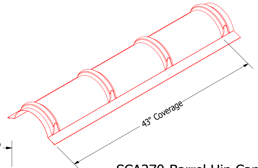
SCA370-Barrel Hip Cap (Standard)
