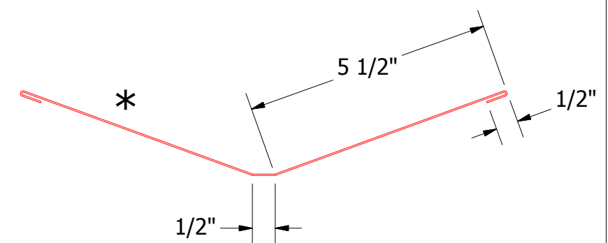
SCA805-Valley Cover
