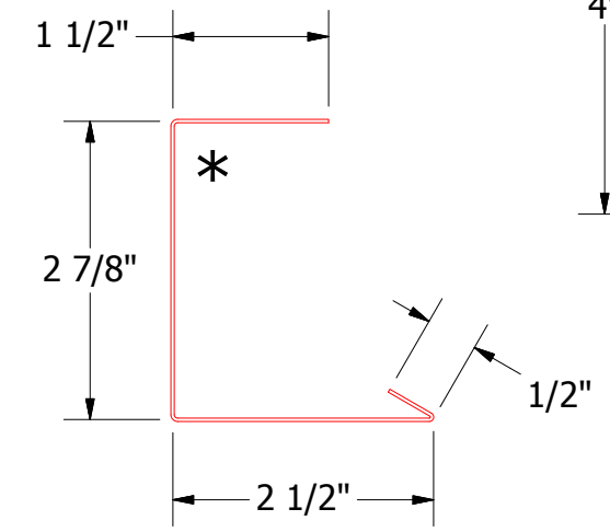
SCA270-J Channel
