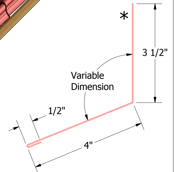
SCA500-Headwall Trim
