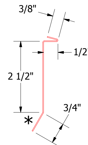
SCA980-Counterflashing
