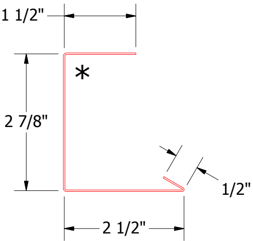
SCA270-Channel Trim
