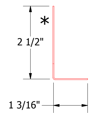
SCA711-Bottom Closure Angle
