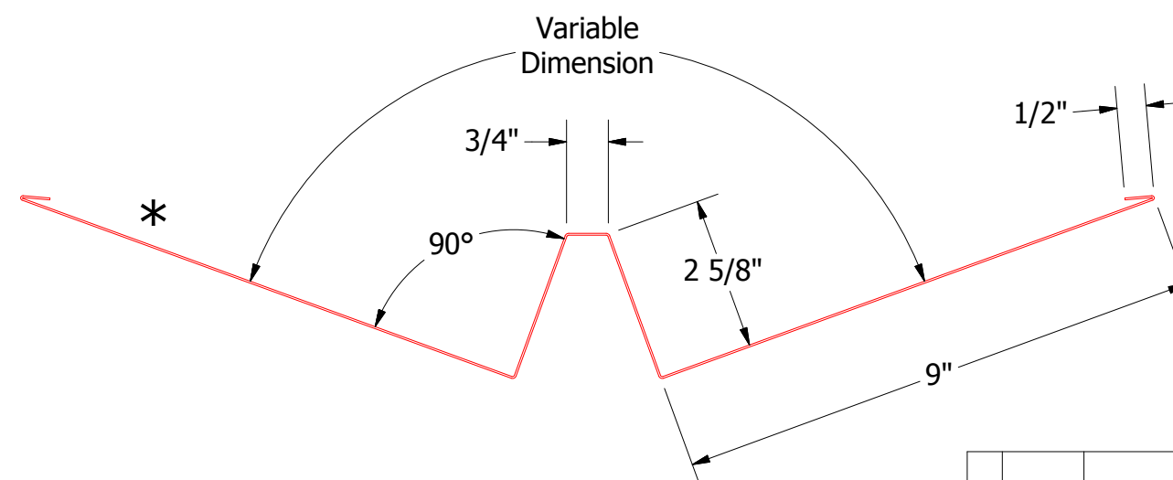
SCA801-Valley Pan
