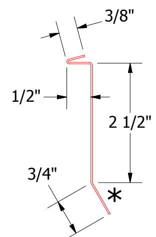
SCA980-Counterflashing
