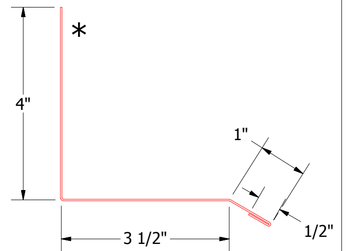
SCA410-Sidewall Trim
